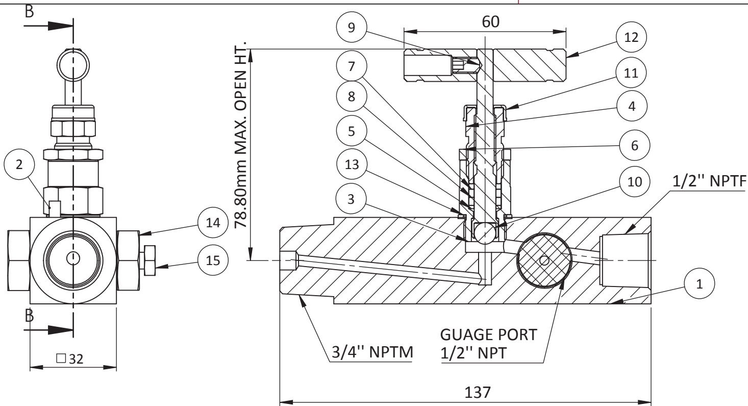
SECTION B-B
