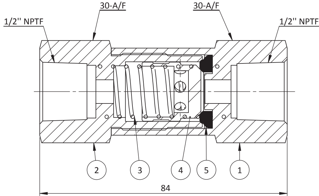
SECTION B-B
